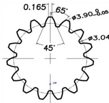
15T 4mm Output Shaft Spline
